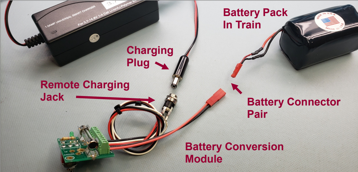
Charging with battery installed in the train
