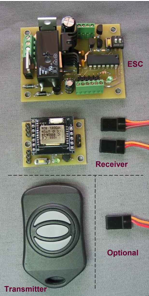
The complete system: ESC (Electronic Speed Control), Receiver & cables, Transmitter, and optional cable for a remote learn button.
